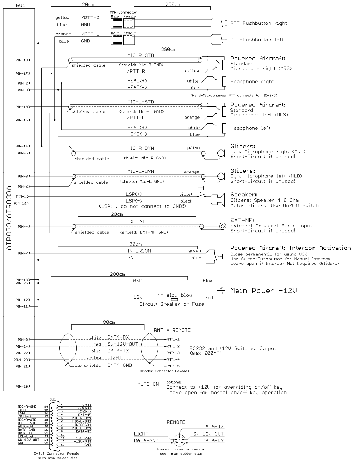
Cable ATR833/ATR833A
